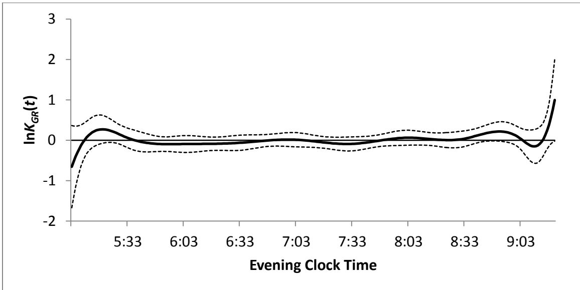
Figure 1. Standard Veil Test Statistic – 8 Internal Knot, 3rd-order Spline
