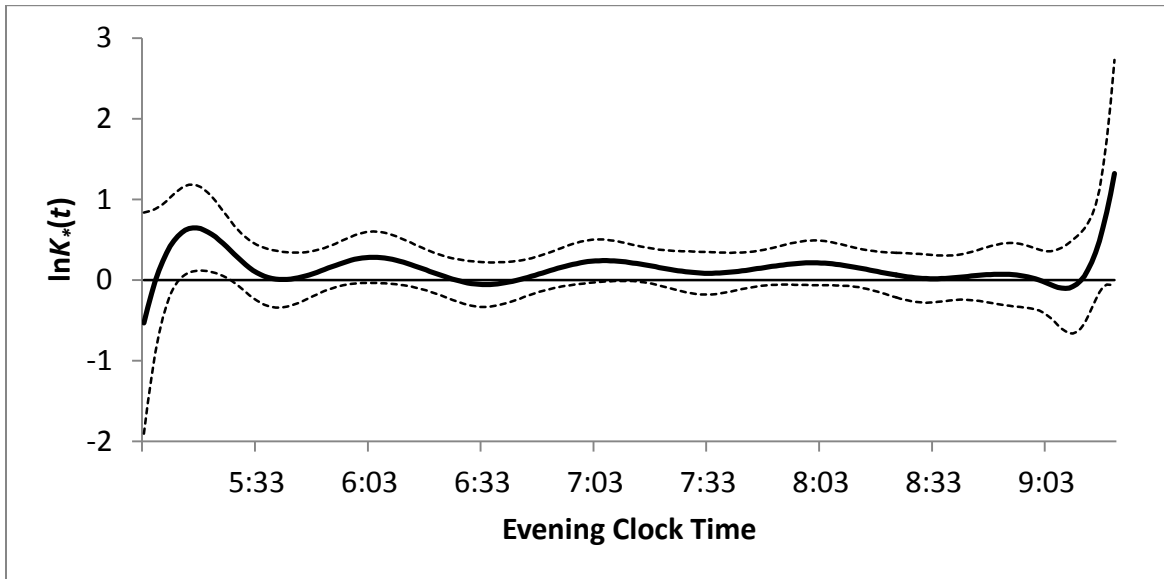
Figure 2. Refined Veil Test Statistic – 8 Internal Knot, 3rd-order Spline
